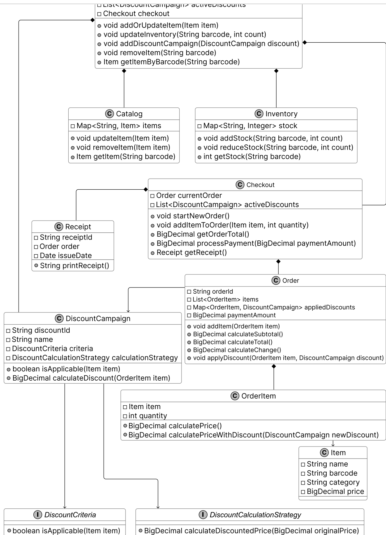
Class Diagram of Grocery Store System
