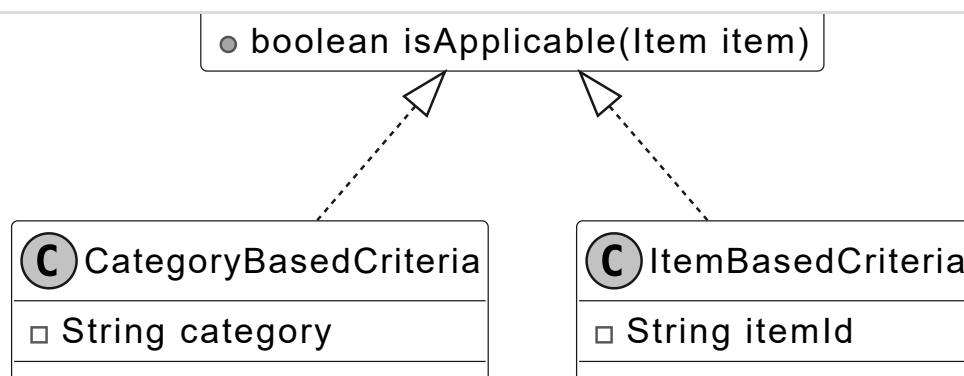
DiscountCriteria interface and concrete classes
