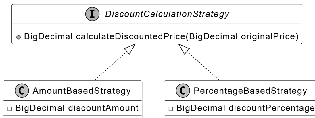
DiscountCalculationStrategy interface and concrete classes
